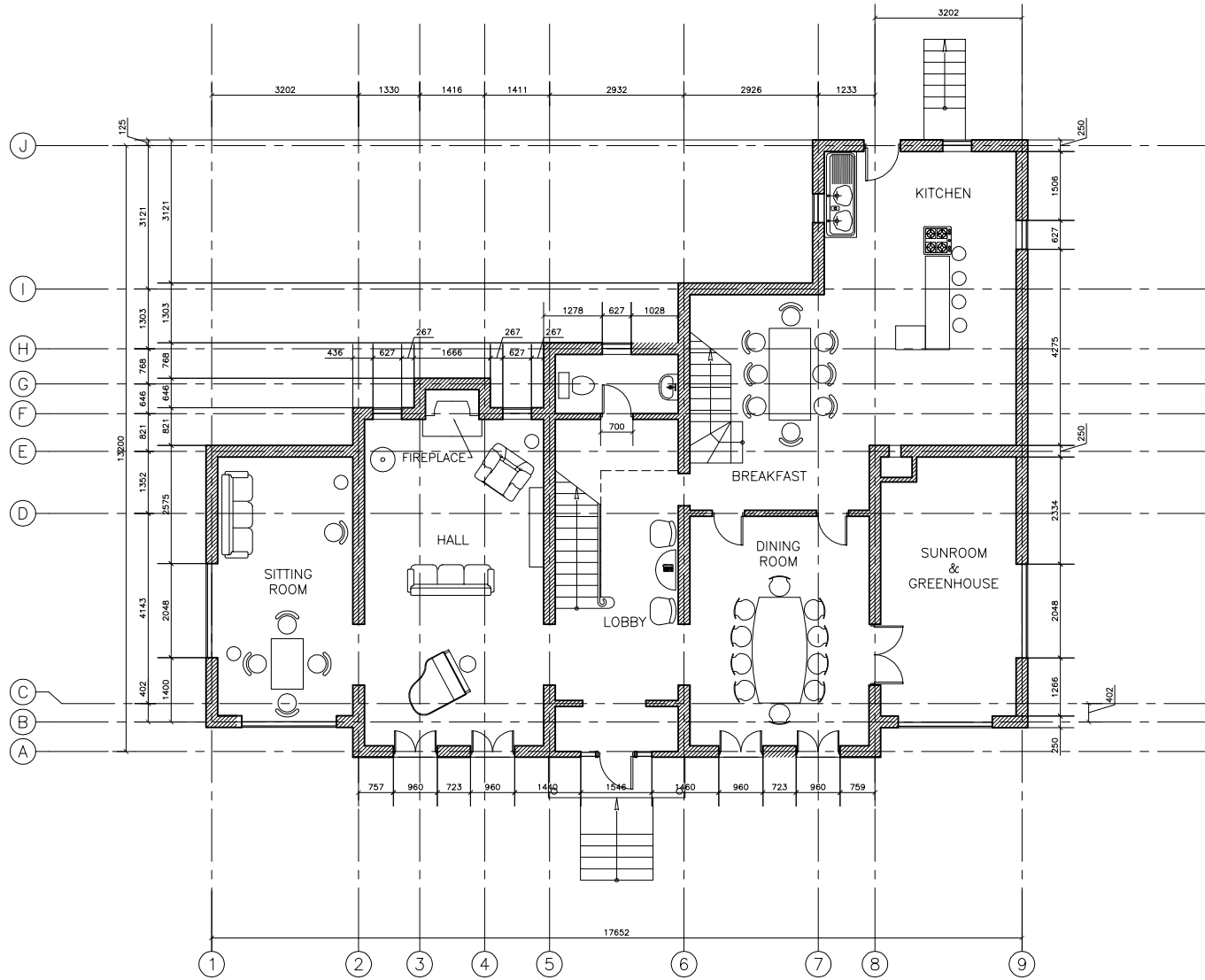
McCallisters' House Ground Floor Plan scale 1:100
